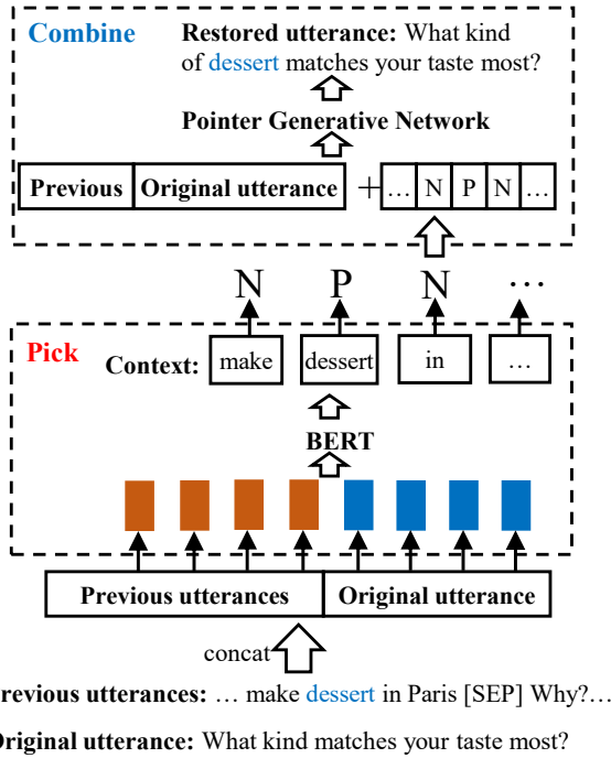
Figure 2: The pick stage predicts which words in previous utterances are omitted by the original utterance. P represents the label of positive, namely the omitted words. In combine stage, the picking result is appended to original conversation as extra guidance for the complete utterance sequence generation.
